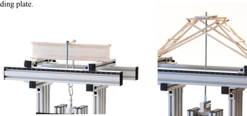
The beam on the left is secured using a U-bolt and quick links while the structure to the right is secured using a threaded rod attached to a metal loading plate.
